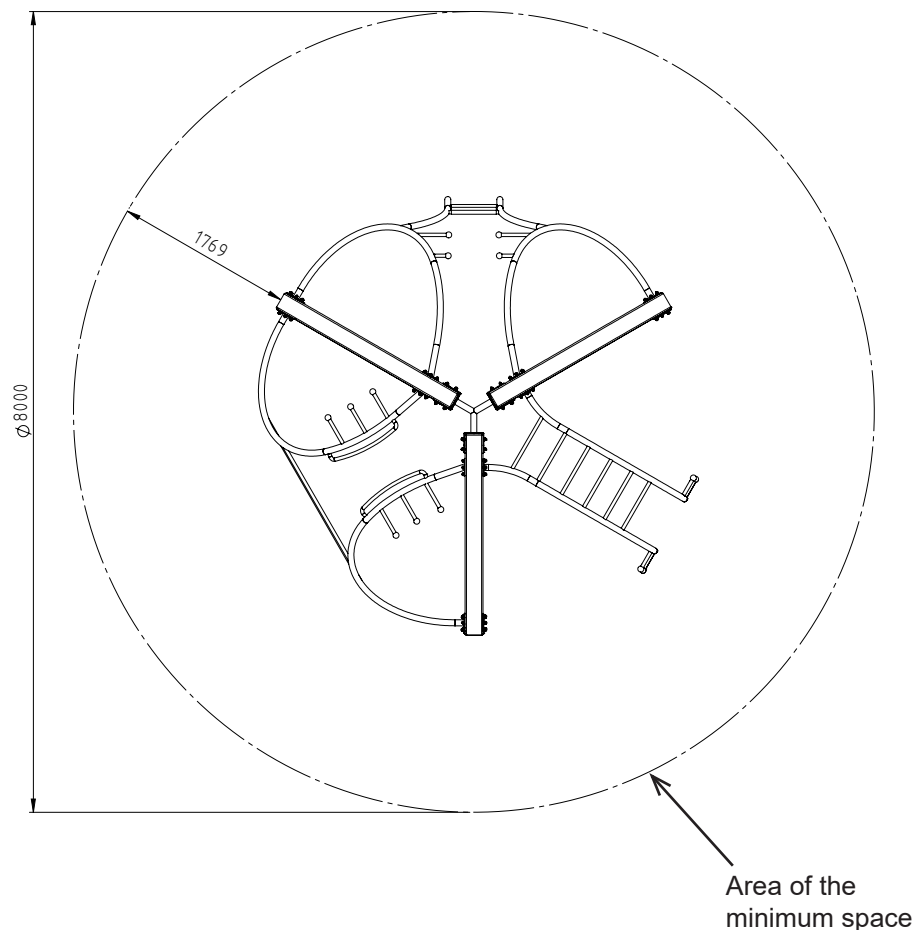
Diagram 4: Top view
