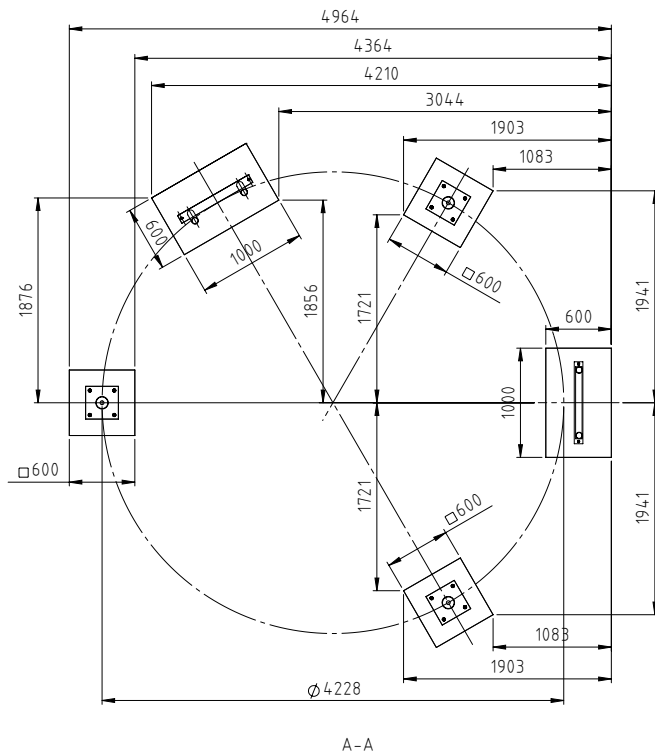
Diagram 2: Foundation plan
